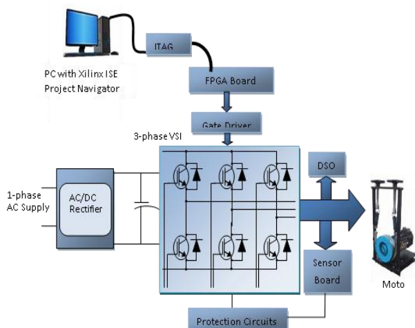
Fig. 7. Hardware implementation
